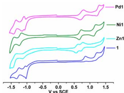
Figure 3. Cyclic voltammograms of 1 , Zn1 , Ni1 , and Pd1 in dichloromethane at 25 °C (scan rate 50 mV/s).
