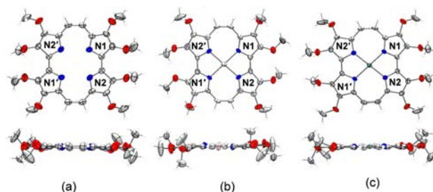
Figure 2. X-ray crystal structure of (a) 1 , (b) Zn1 , and (c) Pd1 (above front view and below side view) drawn in 35% probability level. Color code: C, gray; N, blue; O, red; H, white; Zn, pink; Pd, green.
