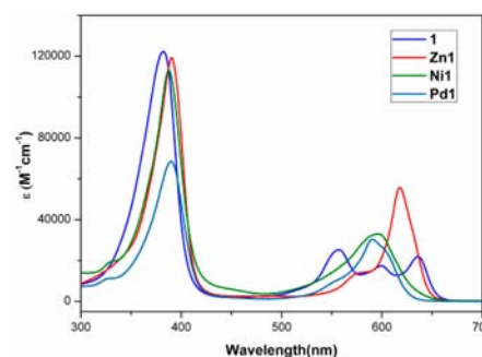
Figure 1. UV-vis spectra of 1 , Zn1 , Ni1 , and Pd1 in chloroform at 25 °C.
